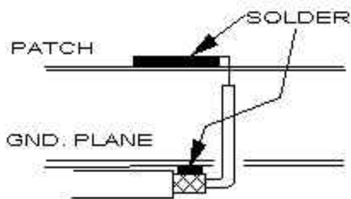
FEED POINT DETAIL
